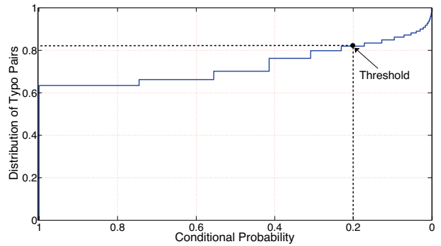
Fig. 3. Conditional probability distribution for user intent modeling.
